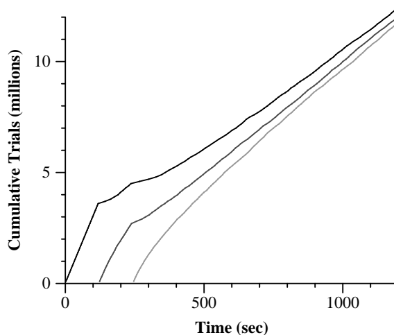
Figure 6: Monte-Carlo Execution Rates. Three identical Monte-Carlo integrations are started two minutes apart. Each task periodically sets its ticket value to be proportional to the square of its relative error, resulting in the convergent behavior. The “bumps” in the curves mirror the decreasing slopes of new tasks that quickly reduce their error.
