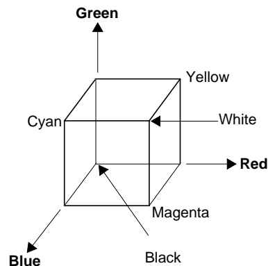
Figure 4-1 The Color Cube in Black and White
